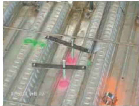
Figure 2: Color coding shows locations for sheet metal straps and pipe hangers on metal decking
